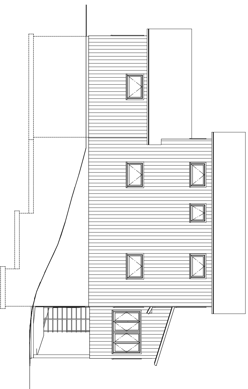
Gelbard Residence Existing Condition Drawing: West Elevation stephen gerard dietemann architect
